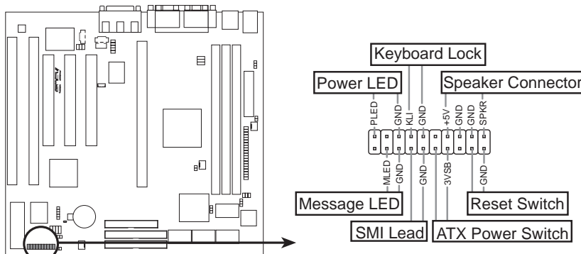
P2L-VM/P2E-VM System Panel Connectors
